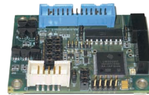
GIO Board
